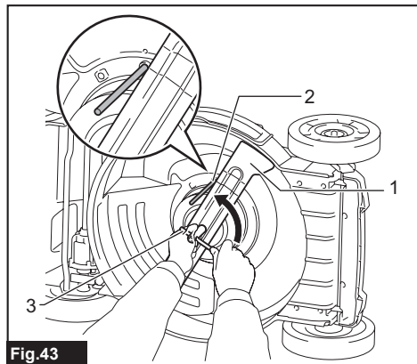
Fig.43 ► 1. Mower blade 2. Pin 3. Box wrench
